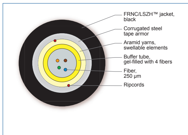
Cross Section of Part Number: 004EEY-13122A2G
