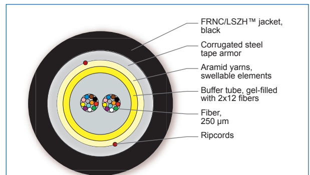
Cross Section of Part Number: 024EEY-13122A2G
